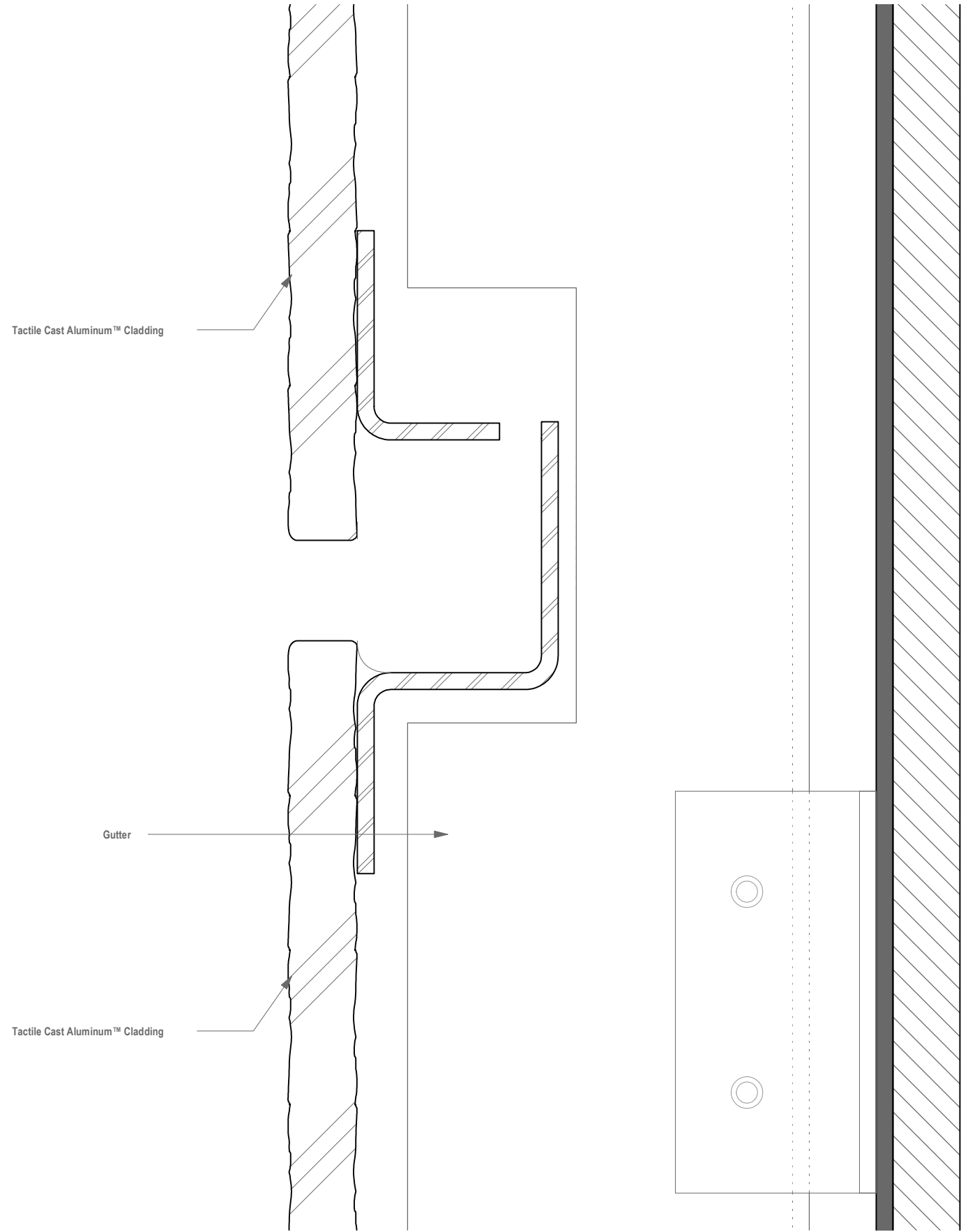
1 Section - Typical Horizontal Joint - Tactile Cast Aluminum™ Cladding M-05 Scale: Full Scale
