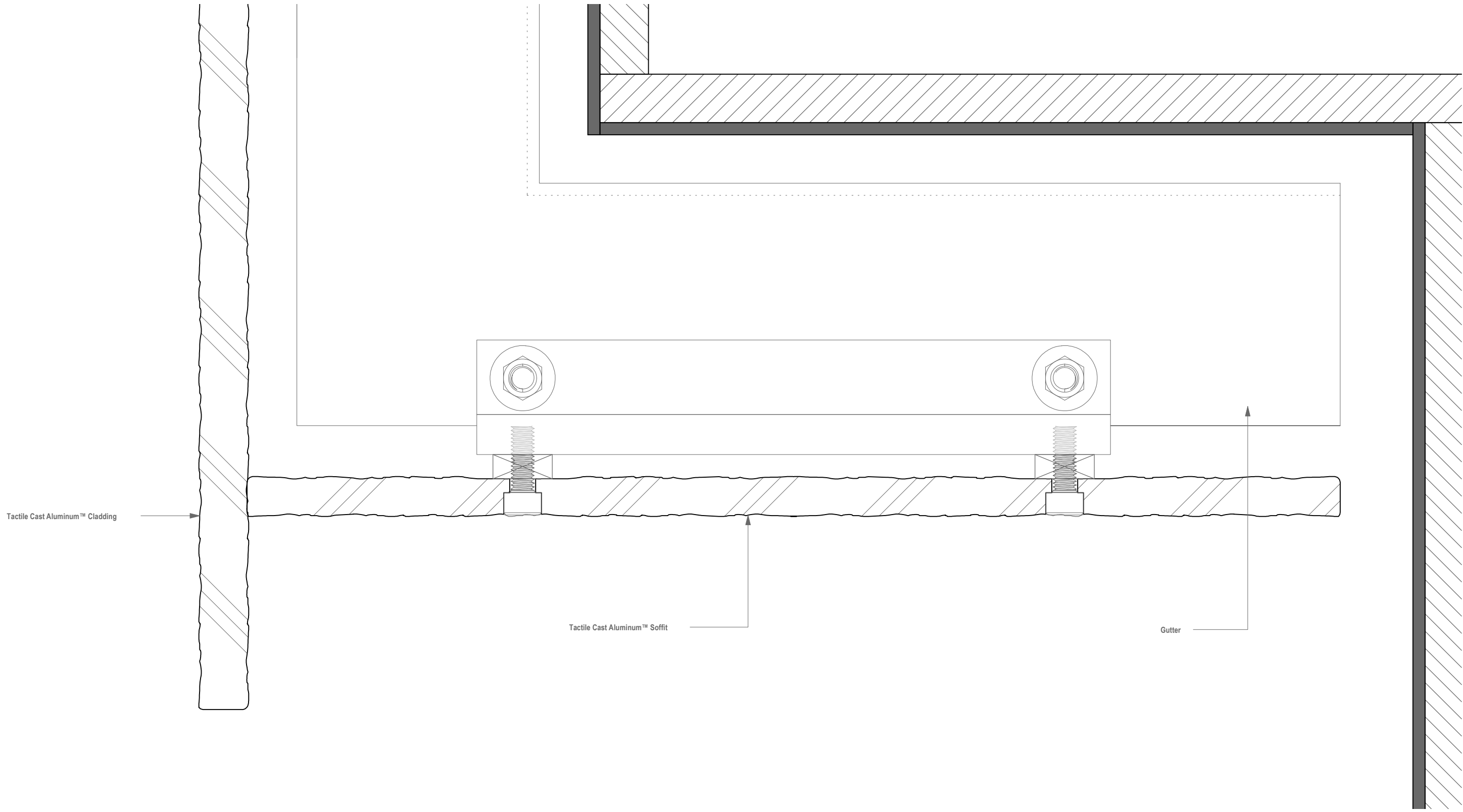
1 Section Detail - Soffit to Vertical Cladding - Tactile Cast Aluminum™ Cladding M-01 Scale: Full Scale
