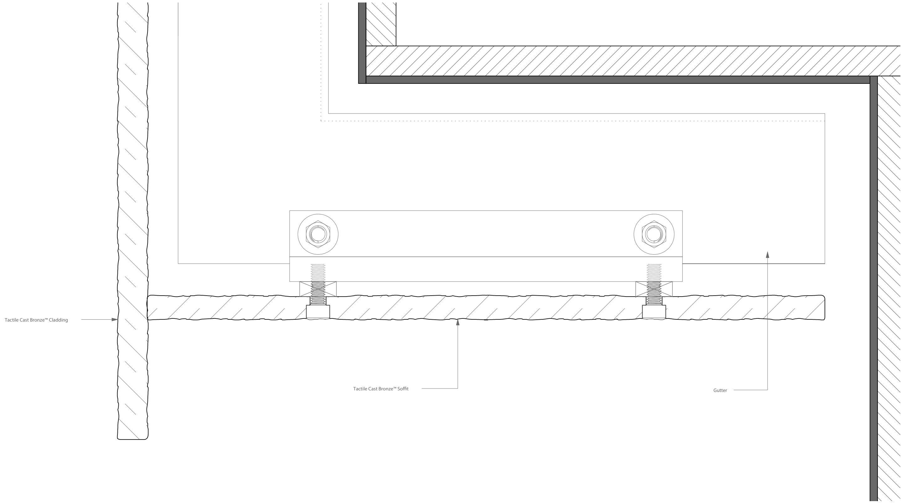
1 Section Detail - Soffit to Vertical Cladding - Tactile Cast Bronze™ Cladding M-01 Scale: Full Scale
